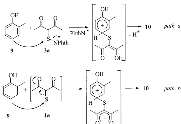
Scheme 3. Possible mechanisms for the formation of sulfide 10
