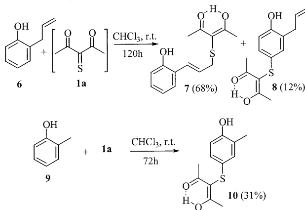
Scheme 2. Reaction of thione 1a with o -allyl phenol 6 and o -cresol 9
