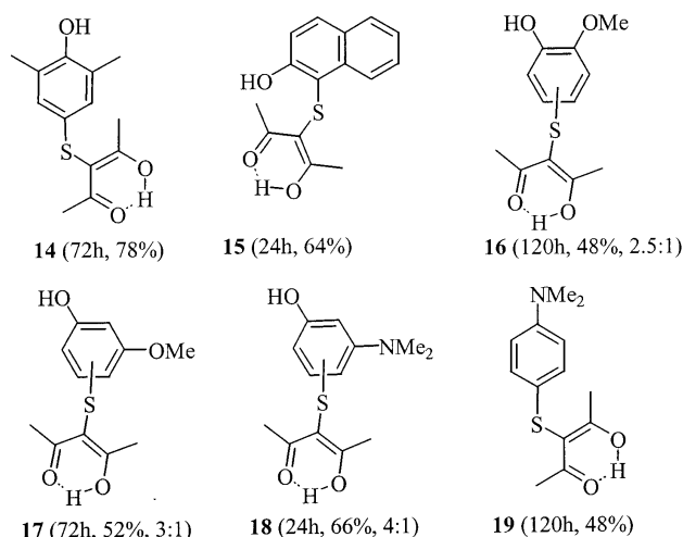
Figure 1. Aryl alkyl sulfides 14–19 obtained by treating thione 1a with phenols and with N,N -dimethylaniline
