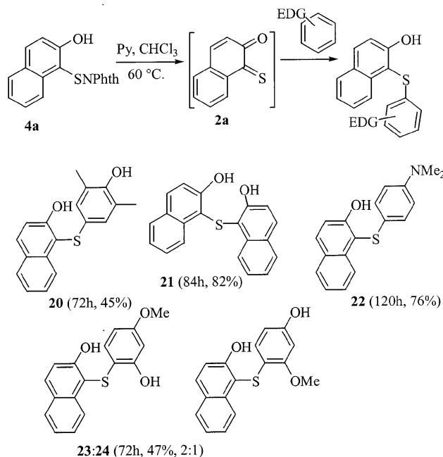
Scheme 5. Diarylsulfides obtained from S_EAr of thioquinone 2a
