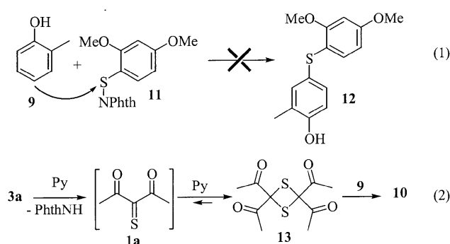
Scheme 4. Evidence for the actual mechanism operative in the formation of 10
