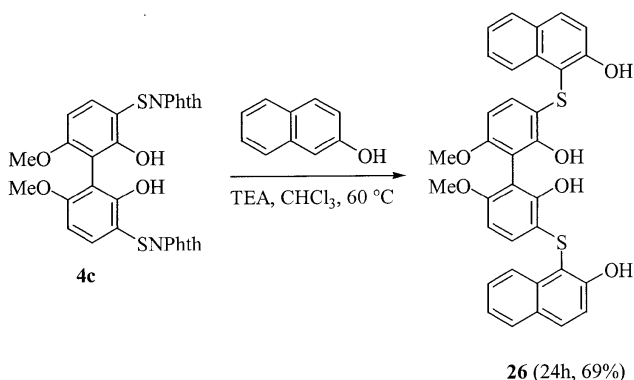
Scheme 7. Synthesis of atropoisomeric biphenyl sulfide 26
