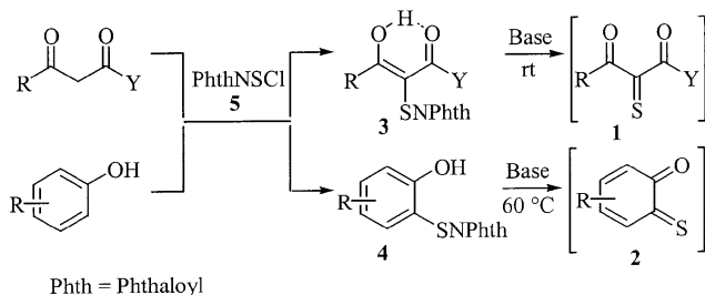
Scheme 1. Generation of \alpha,\alpha' -dioxothiones and ortho -thioquinones
