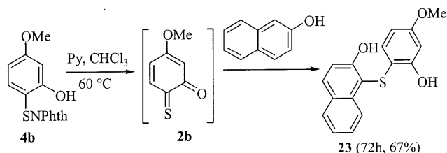
Scheme 6. Reaction of thioquinone 2b with \beta -naphthol
